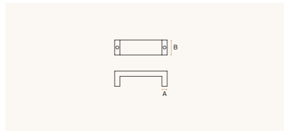
FH17 Material: SUS304 / SUS316 Type: Furniture Handle Available Finishes: SSS / PSS / AB / PC / PVD-SG/PG/SC/CRP/CRS
