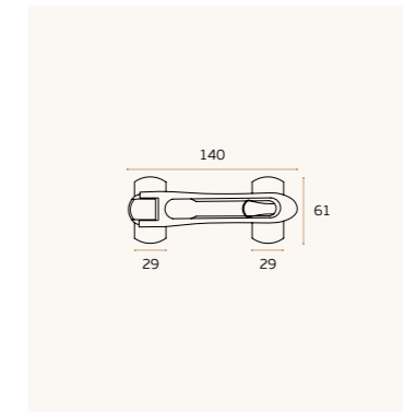
Door Guard
